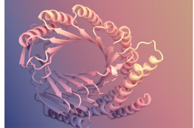
AlphaFold3
